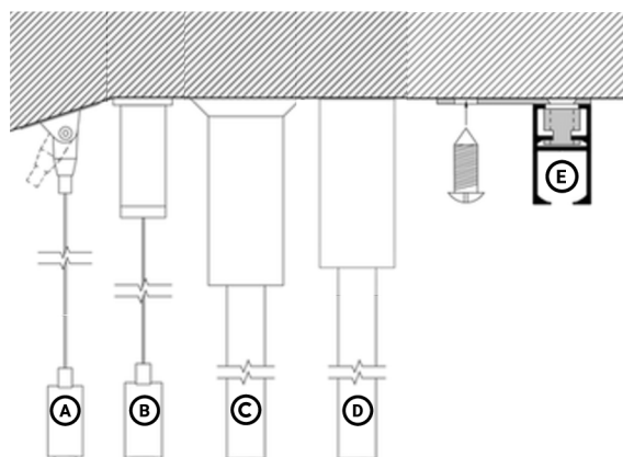
Ceiling Suspension Options
